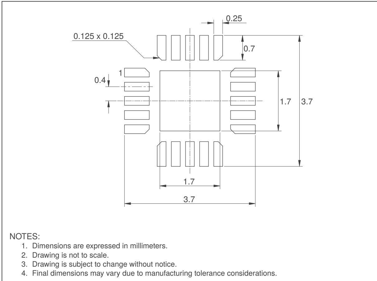
Figure 11.5: QFN20 Recommended Footprint
