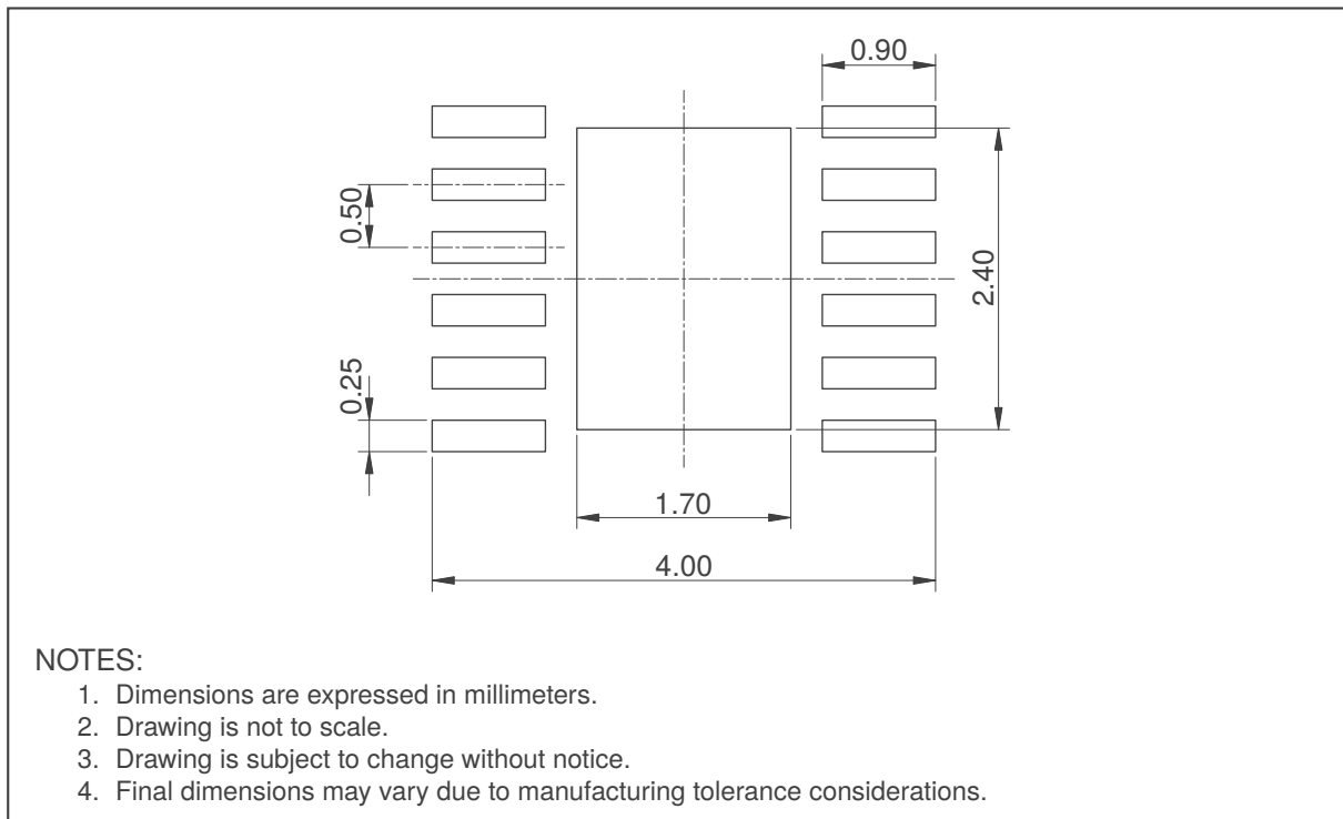
Figure 11.3: DFN12 Recommended Footprint
