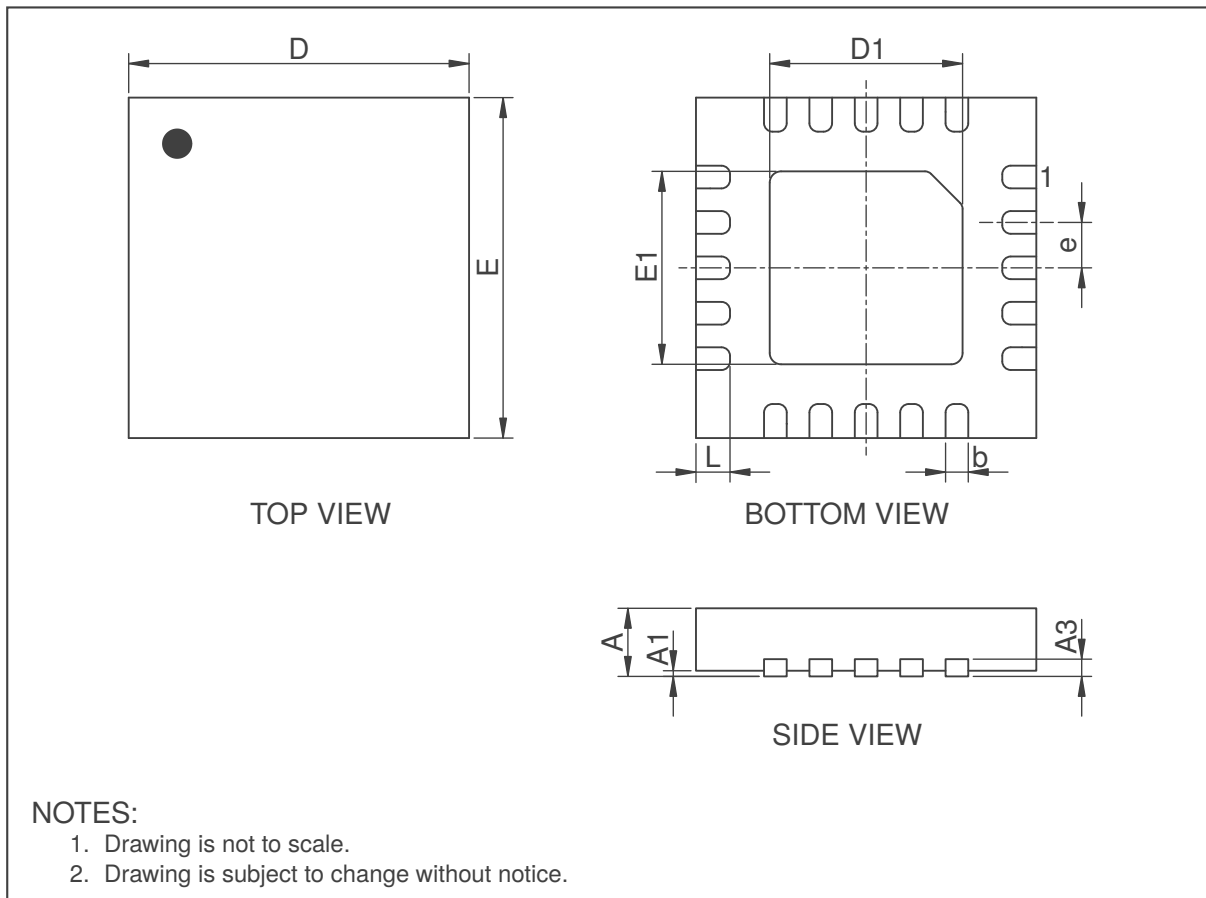
Figure 11.4: QFR (3x3)-20 Package Outline Visual Description
