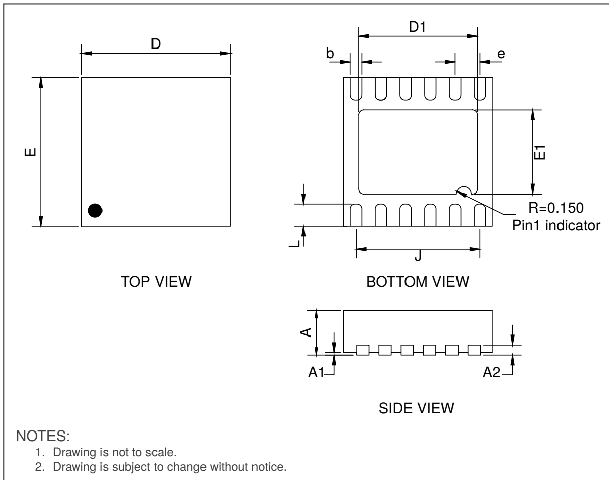
Figure 11.2: DFN (3x3)-12 Package Outline Visual Description
