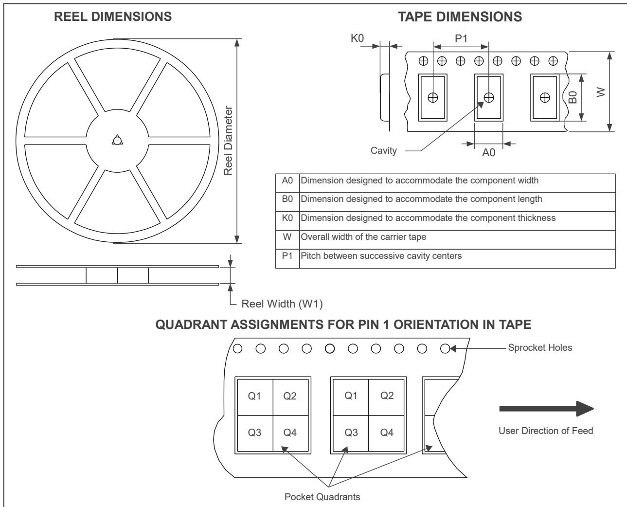
Figure 11.6: Tape and Reel Specification
